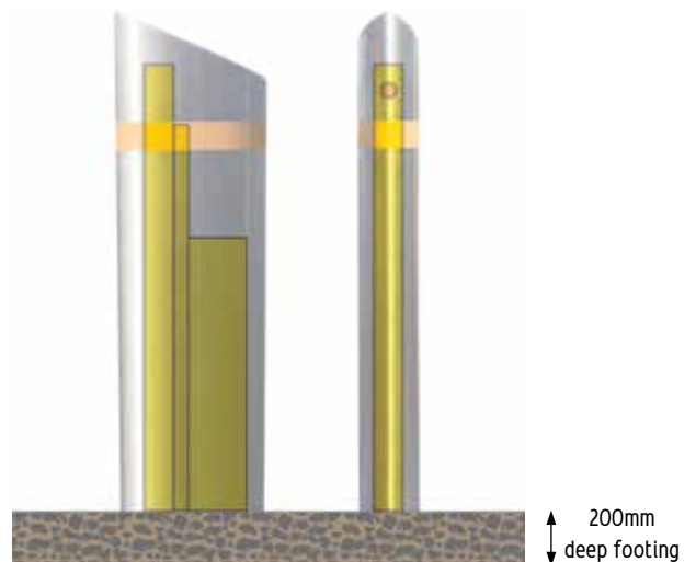
Foundation only 200mm deep x 900mm wide x 1200mm long Tested and passed as a single removable bollard
